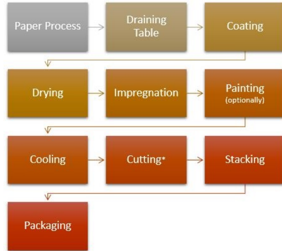
*Cutting for corrugated bitumen tiles
